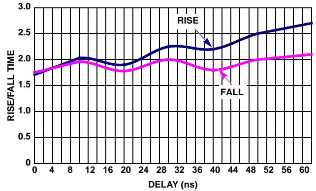
FIGURE 15. ISL59920 RISE/FALL TIME vs DELAY TIME (GAIN = 2)
